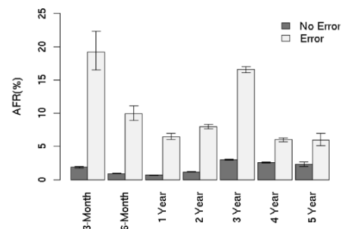
Figure 7: AFR for reallocation counts.
